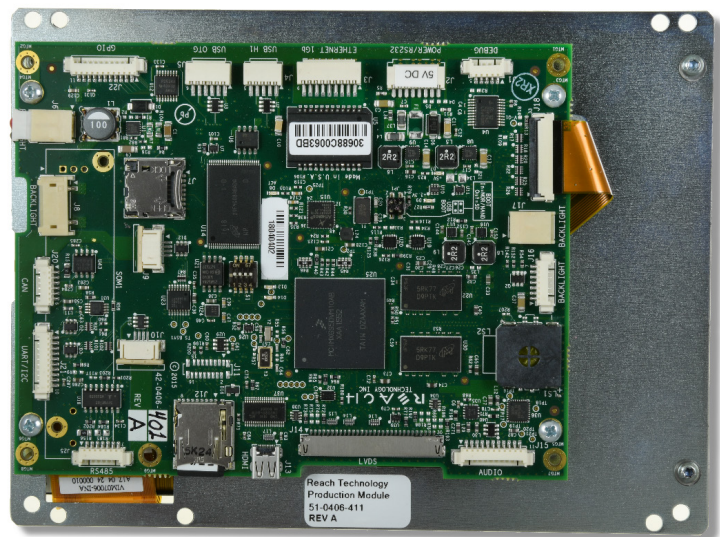
7" G2H2-7R Display Module, back view
