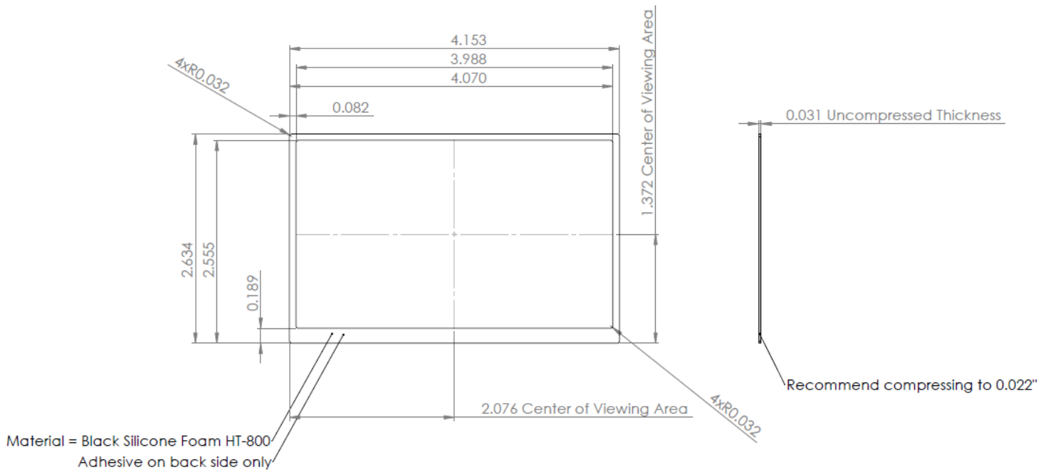
Front and side views with mechanical specifications
