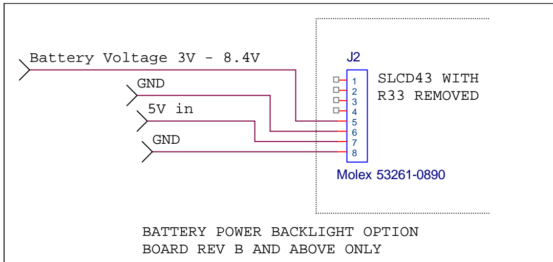
Figure 8: Battery Power Diagram
