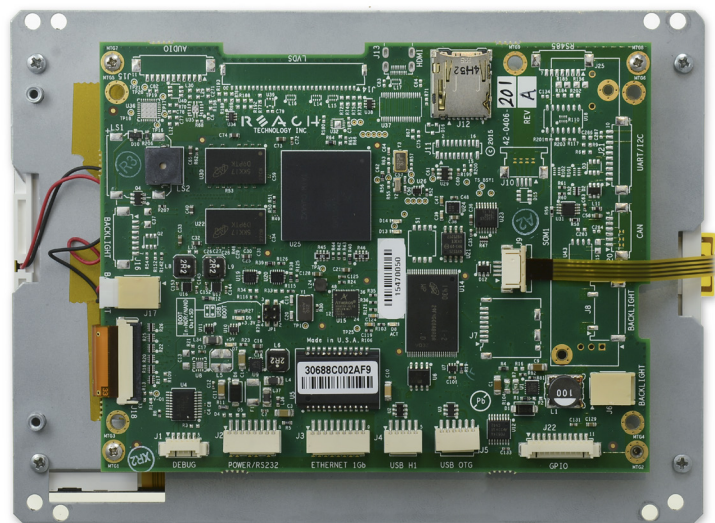
7" G2H2-7R Display Module, back view
